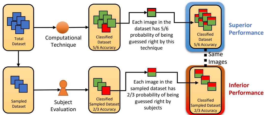
Figure 2.5: Illustration of the performance comparison between computational techniques and our subjects' results. All images used in the test were previously tested by at least one computational technique. Input images from a dataset are represented in blue, and after a testing procedure by a technique (top) or by a subject (bottom), can be rightly classified (green), or wrongly classified (red). Different techniques use different testing methodology and metrics. However, independently of the metric used, they outperform human subjects, which correctly classified the images only approximately half of the time. Note that the numbers used for accuracy in this example ( 5/6 and 2/3 ) are merely illustrative.
