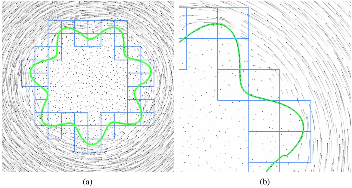
Figure 5.7: Irregularly shaped object example: (a) Gear-like shape with high frequency features, (b) zoomed version of the same example.
