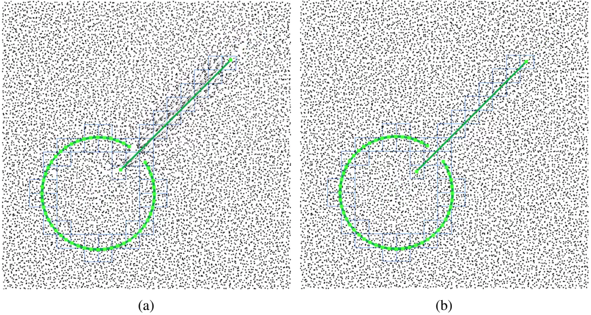
Figure 5.3: No-slip and free-slip stress tests. In this example the line translates tangentially to its geometry: In (a), with no-slip the translation disrupts the flow, since the velocity at the boundary is set to be the solid's velocity. In (b), with free-slip boundaries, the fluid is freely allowed to flow tangentially and no disturbance is shown, as expected.
