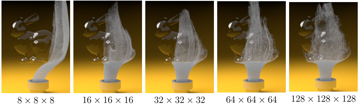
Figure 5.10: Simulation of fluid flow around the Bunny model (free-slip, same time step) using grids of various resolutions. While the level of turbulent detail naturally increases at higher resolutions, the flow still respects the geometry even at extremely coarse resolutions.
