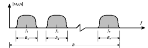
(b) Spectrum of composite baseband modulating signal
