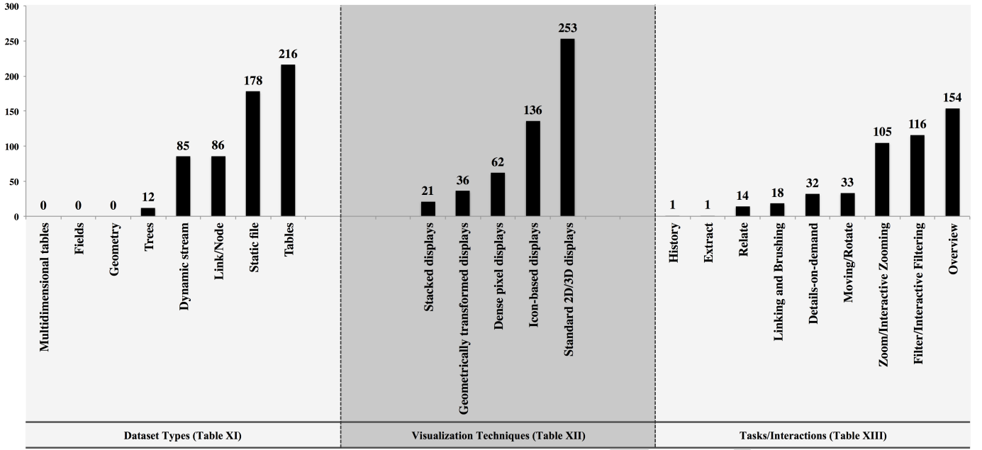
Figure 16. The 285 surveyed articles and papers classified following the information visualization taxonomy. Each topic of the taxonomy is identified in the bottom of the chart, together with the reference to its table in Appendix C. Moreover, subtopics are separated by dashed lines. Black bars depict the number of articles and papers classified in the taxonomy subtopics.
