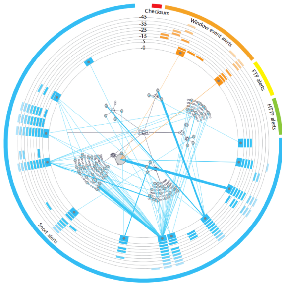
Figure 10. VisAlert visualization [102]. In the center of the circle is a graph layout of the network. The circle's radial sections moving from most recent (closest to the topology map) to the least recent. The outside circular element determines the alert type.
