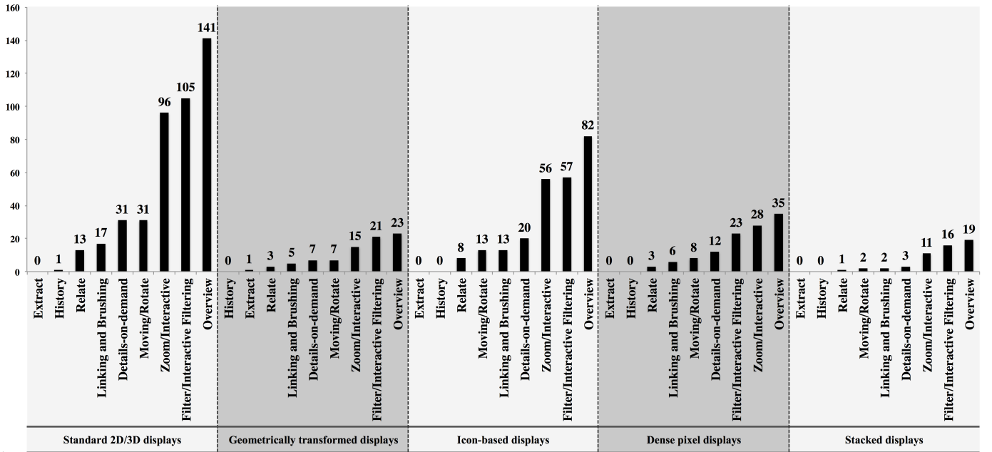
Figure 17. A classification that shows how tasks/interactions subtopics appear together with subtopics of the visualization techniques topic. Each subtopic of visualization techniques is identified in the bottom of the chart. Moreover, visualization techniques subtopics are separated by dashed lines. Black bars depict the number of articles and papers that use each subtopic of the tasks/interactions topic.
