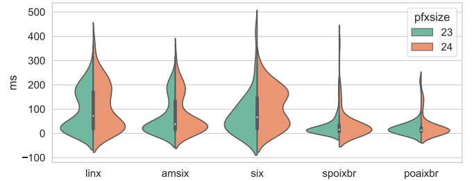
Fig. 2: More specific prefix impact on RTT
