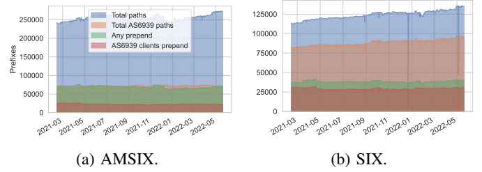
Fig. 7: The impact of AS6939 on IXP routing table.
