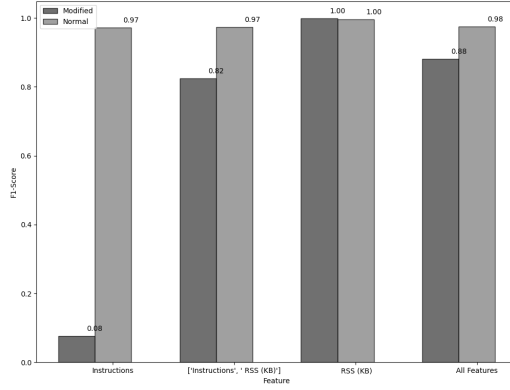
Fig. 3 F1-score for the Detection of Anomalous Traffic using Different Features
