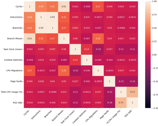
Fig. 2 Heatmap for Metrics Correlation and Selection
