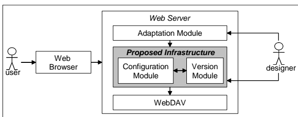
Figure 1: Content server architecture
