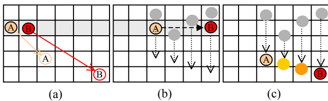
Figure 11. Pipelined reconstruction: (a) Two adjacent texels and their final positions. (b) and (c) Horizontal and vertical interpolation interspersed.
