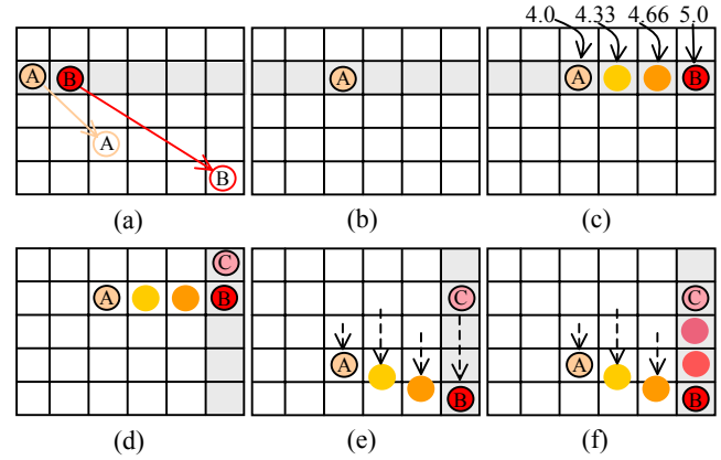
Figure 8. Warping of one texel. (a) Source texels A and B and their final positions after the warp. (b) The first texel of the current row is moved to its final column. (c) Next texel is moved to its final column and color and final row coordinates are interpolated during rasterization. (d) After all rows have been warped, texel C is adjacent to texel B . (e) Along each column, texels are moved to their final rows. (f) Color is interpolated during rasterization.
