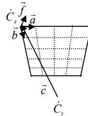
Figure 6. Parallel and perspective projection cameras sharing the same image plane (origin, \vec{a} and \vec{b} vectors).
