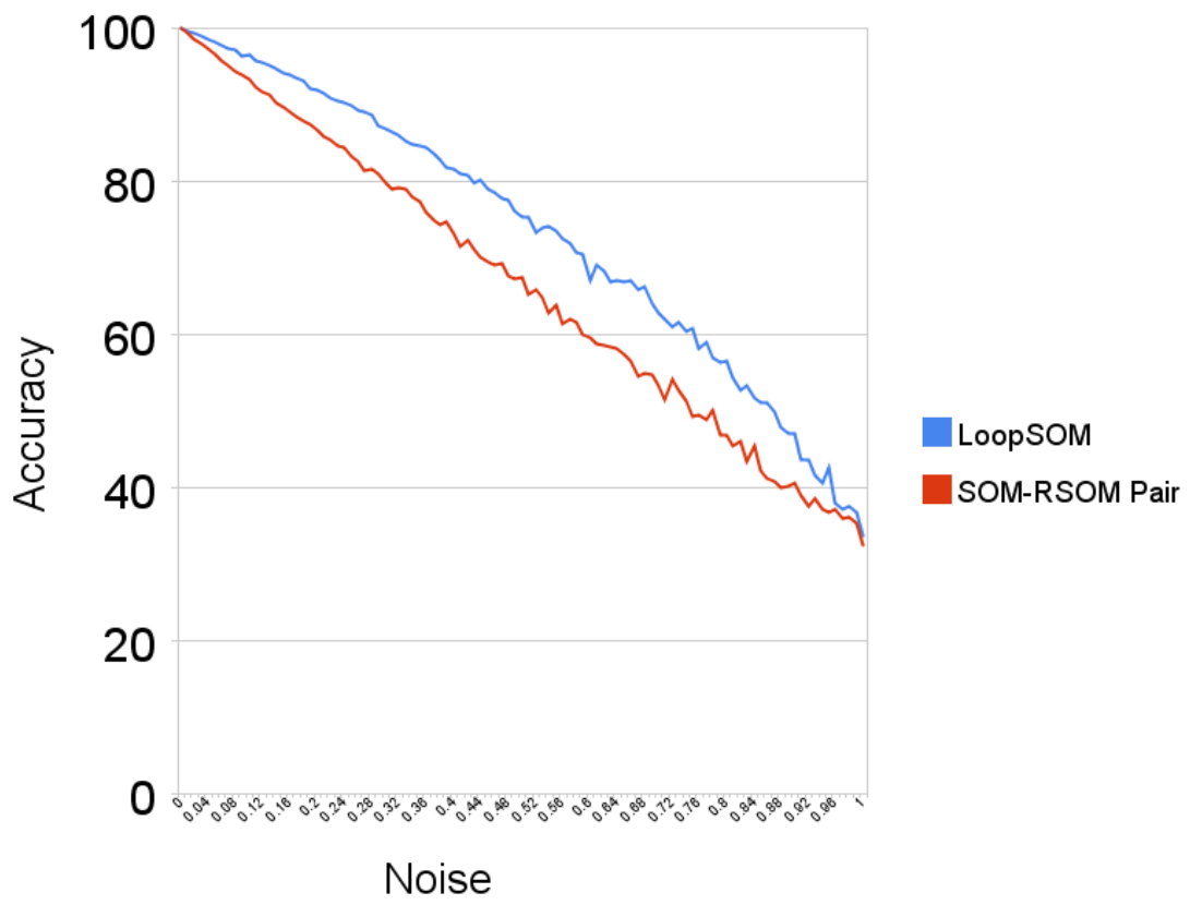
Figure 7. Results comparing the SOM-RSOM pair and the LoopSOM accuracy on a 2D line classification task.
