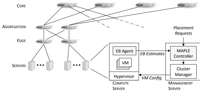
Fig. 2: The MAPLE system architecture. MAPLE is comprised of Effective Bandwidth agents (EB Agents) residing in each server and a MAPLE Controller residing in a management server. EB Agents send effective bandwidth estimates upon request to the MAPLE Controller. The MAPLE Controller processes VM placement requests from tenants and instructs the Cluster Manager, which in turn configures VMs on the selected servers. Whilst the figure illustrates a Fat Tree datacenter topology (see Portland [22]), MAPLE is agnostic of the topology since it collects bandwidth estimates at servers only.
