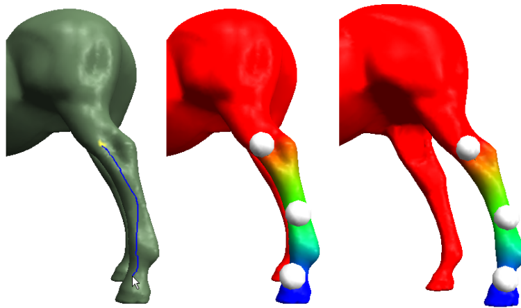
Figure 3.3: Mesh segmentation when two parts of the object project to the same portion of the image plane. Left: Two legs of the Horse model project to the same portion of the image plane. Center: The mesh segmentation algorithm can deal with such cases. Right: The same scene seen from a different viewpoint after region segmentation. Note that just the leg that was nearest to the view plane has been selected and used to create the curve.
