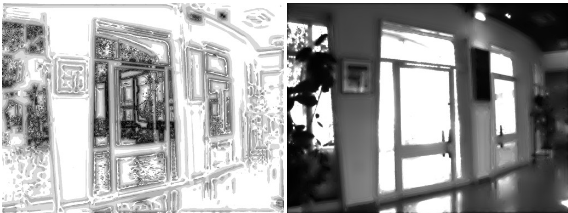
Figure 7.10: The representation of the size of the maximum approximately isoluminant neighborhood of each pixel ( s_{max} ). White means bigger neighborhood. The image on the right shows the estimated local contrast of each pixel ( V(x, y, s_{max}) ). This values will be used to perform dynamic range compression (Equation 4.8). Results obtained using box-filtering, according to the images from Figure 7.8 and 7.9. Note the similarities with the ones using Gaussian filters from Figure 4.10.
