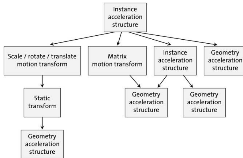
Figure 4.2 – An example of acceleration structure tree, showing possible connections between nodes.
