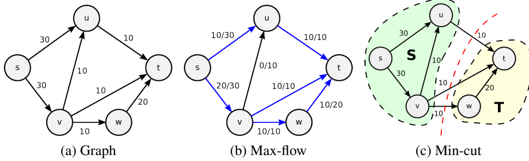
Figure 3.1: Example of a weighted directed graph G with five nodes and seven edges (a). Optimal max-flow for G using s as source and t as sink (b), where the values on the edges represent "flux/capacity". Optimal min-cut for G , dividing it into two subsets S and T (c). Note that the cut (in red) passes right through the saturated edges in (b).
