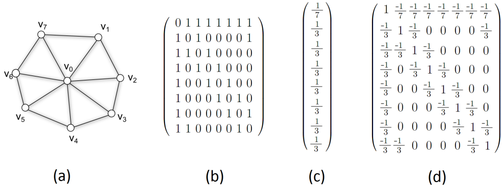
Figure 2.5: Laplacian Coordinates. (a) Polygonal Mesh. (b) Adjacency Matrix A (c) Diagonal of Matrix D^{-1} (d) Laplacian Operator
