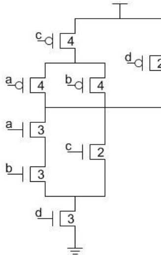
Figure 4.11: CMOS complex gate, with different transistor sizing, according to the Logic Effort (SUTHERLAND, 1999).
