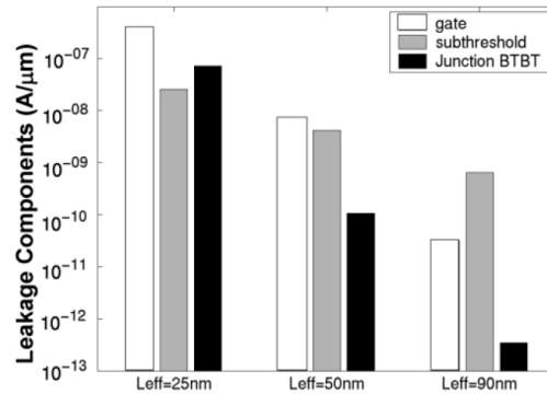
Figure 4.6: Contribution of different leakage components in NMOS devices at different technology generation (MUKHOPADHYAY, 2005).
