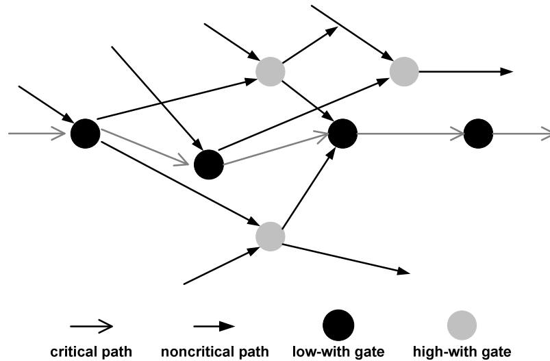
Figure 2.4: Dual V_{th} CMOS circuit (ROY, 2003).
