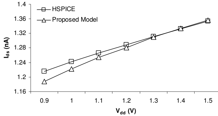
Figure 3.13: Variation of subthreshold leakage current in terms of power supply voltage variation.
