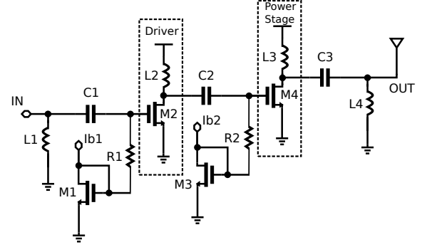
Fig. 1. Topology of proposed PA
