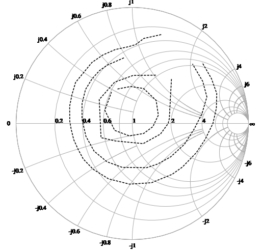
Fig. 2. Load Pull Contours example for 2.4 GHz
