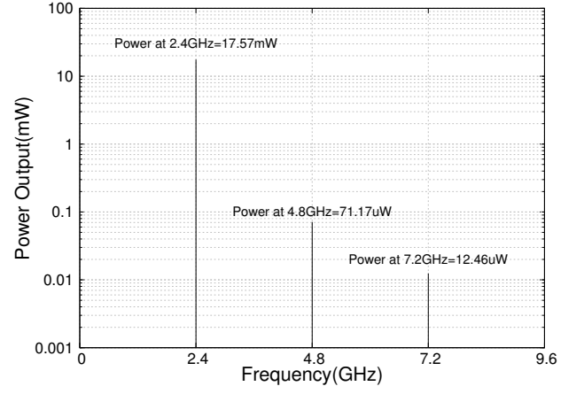
Fig. 5. Spectrum of Output Power
