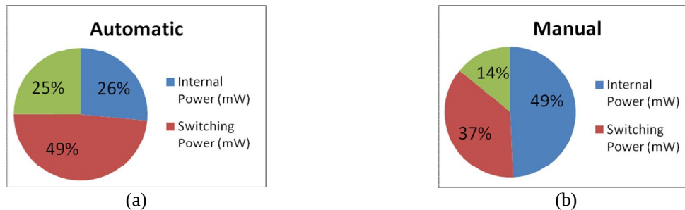
Fig. 3 – Power consumption distribution for the RSA cryptographic cores designed with manual and automatic design flows for the multiple cryptographic operations scenario.
