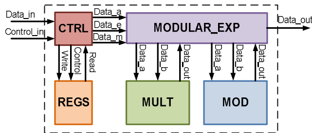
Fig. 2 – Asynchronous RSA cryptographic circuit block diagram. Each arrow represents a handshake channel.
