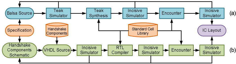
Fig. 1 – Asynchronous circuits design flows, fully automated (a) and manual (b).
