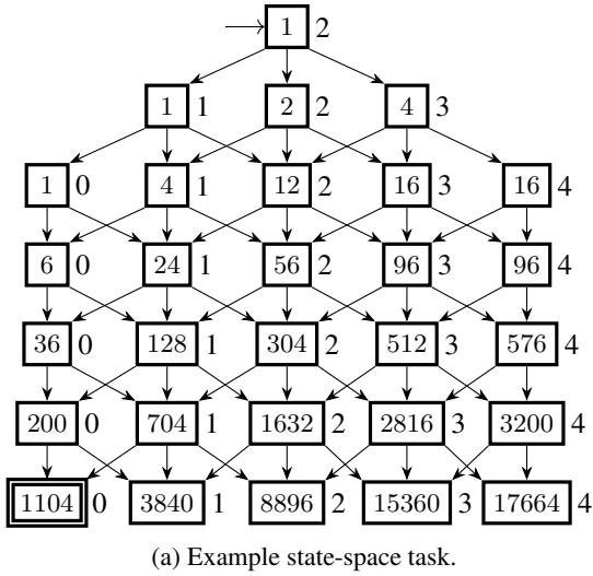
Figure 1: On the left: an example of a state-space task. Each rectangle is a node-set that contains nodes with the same g and h -values. The number at the right of a node-set is its nodes h -value, while the number inside is its size. The depth of a node-set is its nodes g -value. Node sets with nodes g -values greater than 6 are omitted. On the right: an illustration of the node composition of the A^*+IDA^* and PEA^*+IDA^* 's Open lists.
