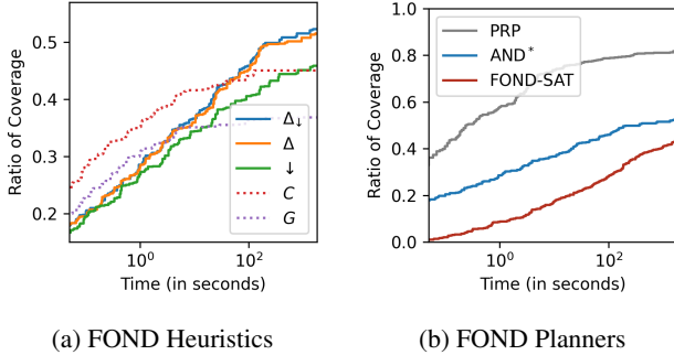
Figure 5: Ratio of Coverage per Time
