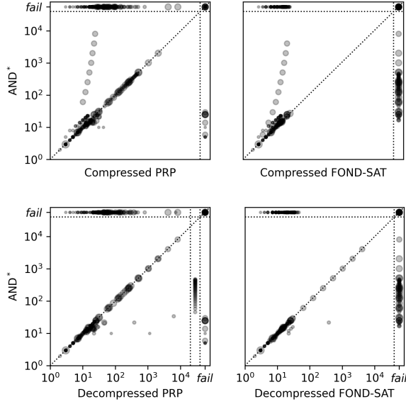
Figure 6: Comparison of Solutions Sizes
