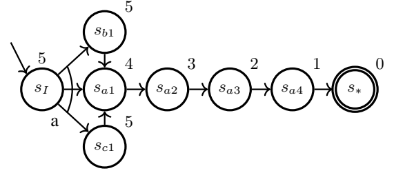
Figure 1: State-Space 1
