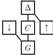
Figure 2: Hasse Diagram of FOND Heuristics Dominance
