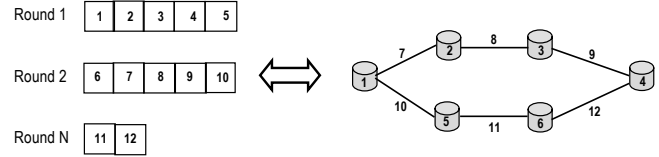
Fig. 3. Allocation windows and rounds
