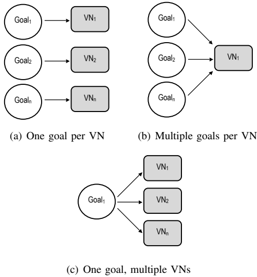
Fig. 2. VN allocation procedures
