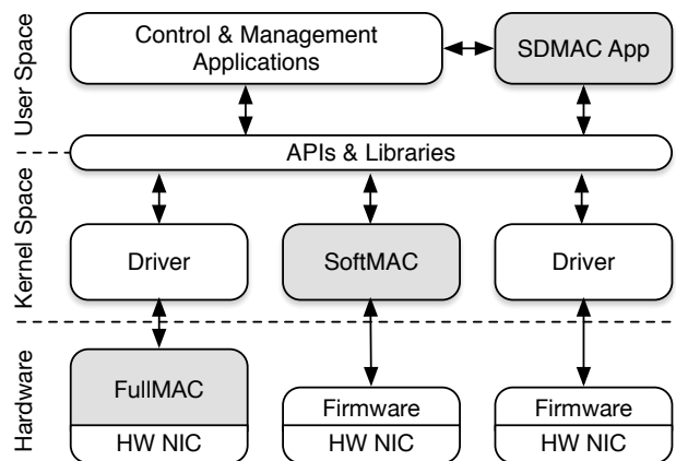
Fig. 4. Programmability scope along with a generic Linux kernel architecture.
