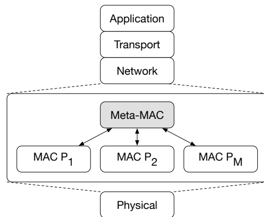
Fig. 5. The Meta-MAC protocol architecture in a simplified protocol stack, Farago et al. [15].
