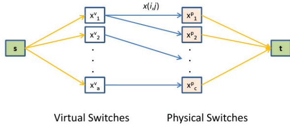
Fig. 3. Graph of min-cost flow problem for switch mapping.
