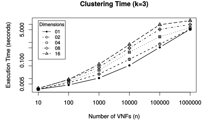
Fig. 7: Time to discover 3 clusters in different scenarios
