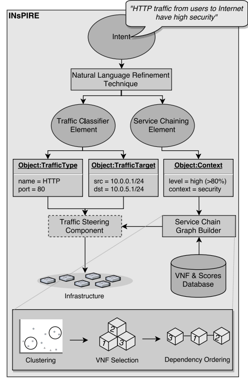
Fig. 3: INSPIRE Intent Refinement Flow
