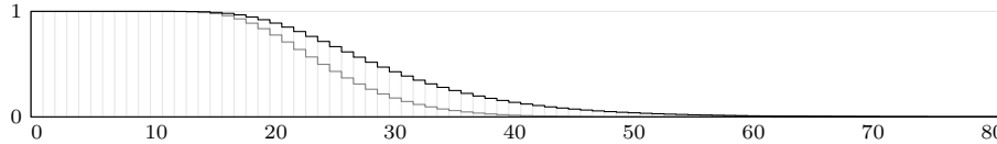
Fig. 45. Random 3SAT on 5 variables when the clauses are sampled with replacement. The probabilities \hat{q}_m are shown with a black line; the smaller probabilities q_m of Fig. 40 are shown in gray.
