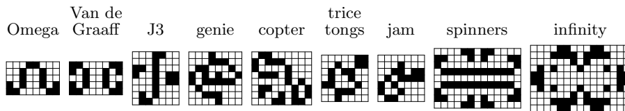
Fig. A-6. Noteworthy minimal oscillators of periods 2 and 3.
