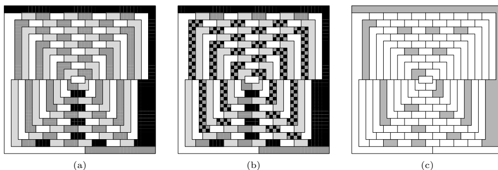
Fig. A-5. Colorings and kernels of McGregor's graph.
