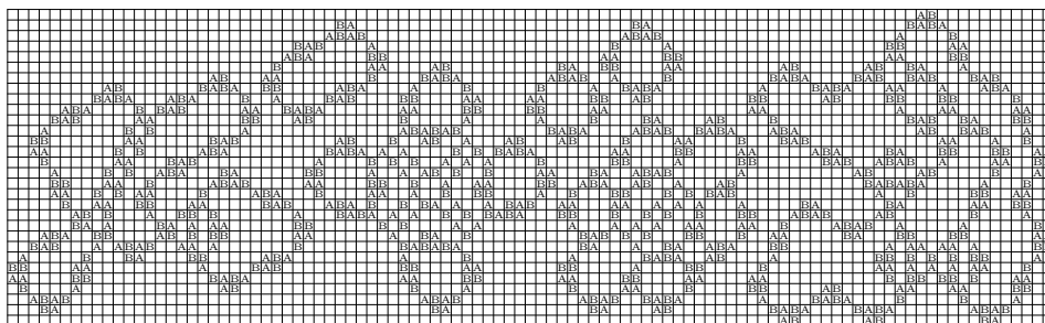
Fig. A-7. Mobile flipflops: An ideal way to tile the floor of a workspace for hackers.
